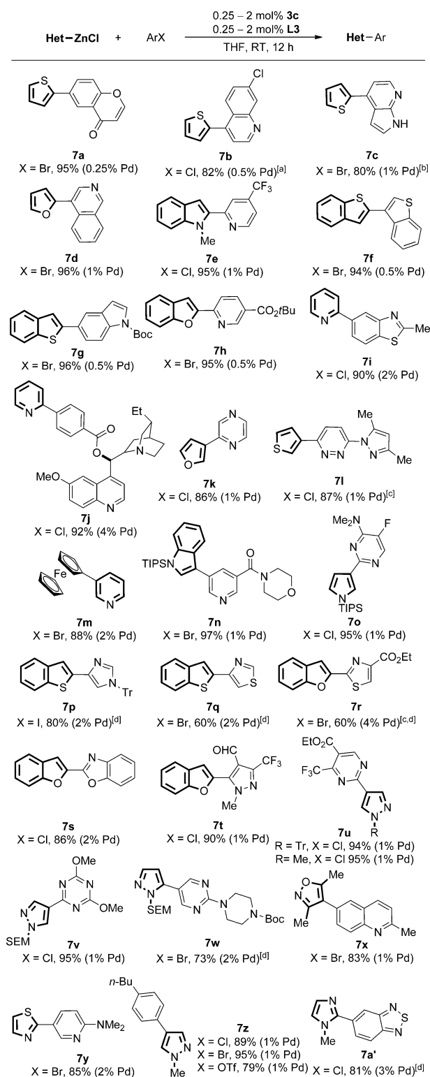
Scheme 2. Cross-coupling of heteroaryl zinc reagents and heteroaryl halides. Reaction conditions: ArZnCl (1.3 mmol), ArX (1.0 mmol), 3c (0.25–2 mol%), L3 (0.25–2 mol%), THF, RT, 12 h. Yields are of the isolated products, and an average of two runs. [a] ArZnCl (1.2 mmol) was used. [b] ArZnCl (2.3 mmol), ArX (1.0 mmol), 3c (1 mol%), L3 (1 mol%), THF, RT, 12 h. [c] 3b and L1 instead of 3c and L3 ; [d] ArZnCl (1.3 mmol), ArX (1.0 mmol), 3c (2–4 mol%), L3 (2–4 mol%), THF, 80 °C, 12 h.
